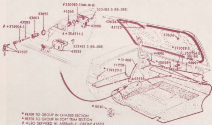
LUGGAGE COMPARTMENT DOOR LATCH and RELATED PARTS 1965/66 MUSTANG - BODY TYPES 65, 76
