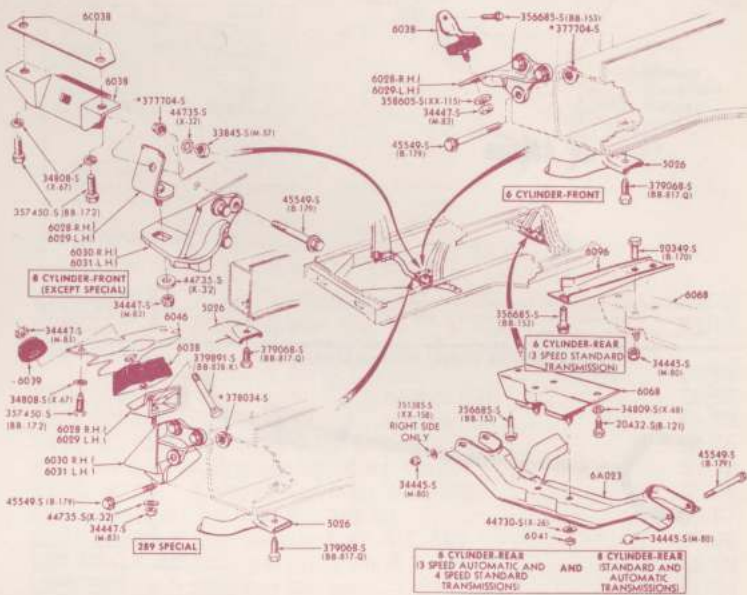
ENGINE SUPPORTS, INSULATORS and RELATED PARTS - FRONT and REAR 1965-68 MUSTANG - 6 CYLINDER 170, 200 and 8 CYLINDER 260, 289
